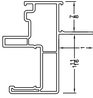
7/8" NFS Frame
